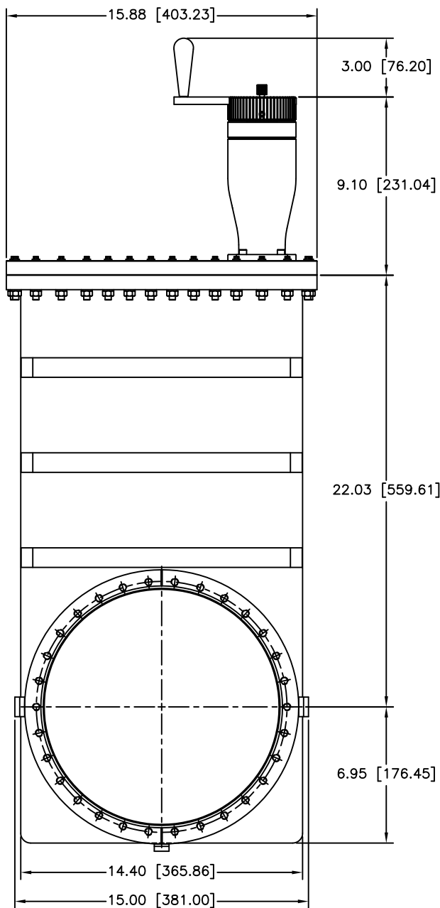
CARRIAGE SIDE
