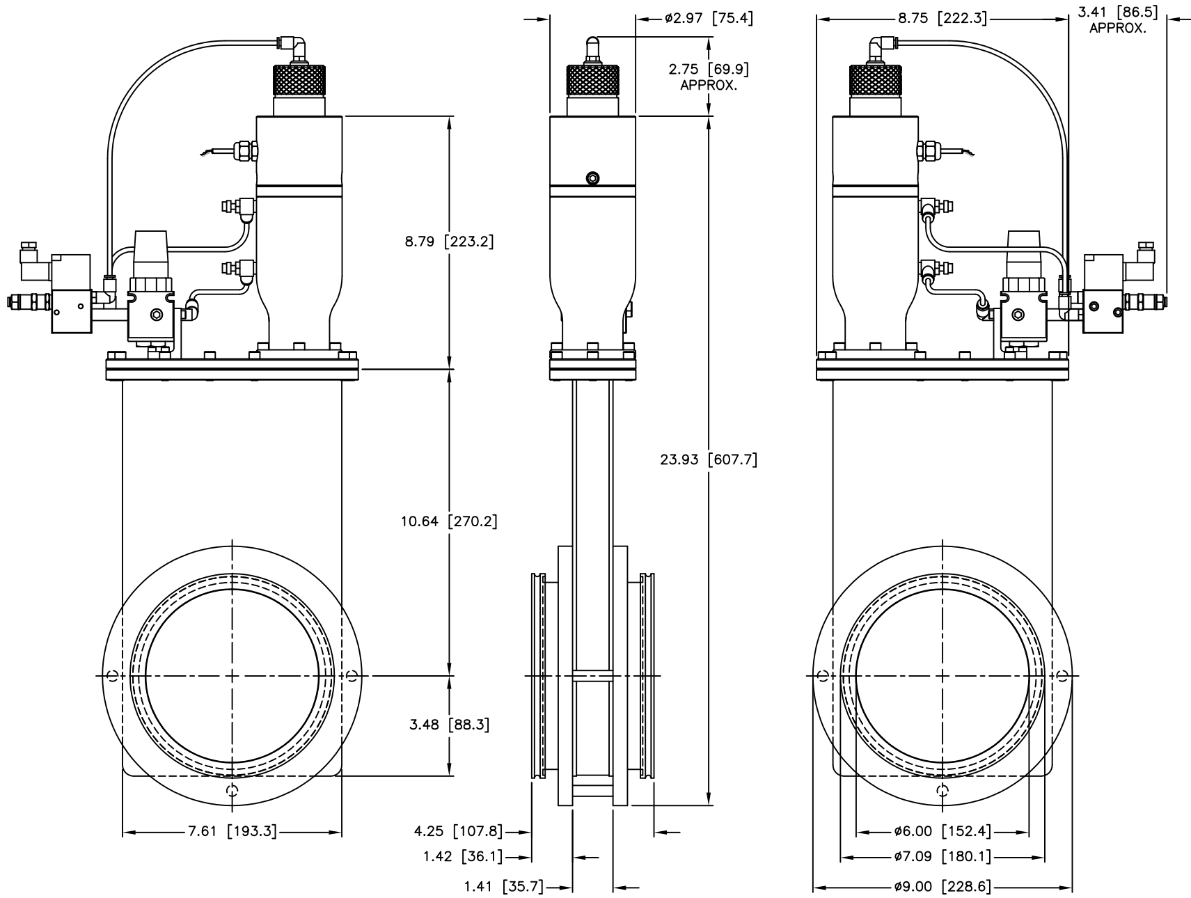
CARRIAGE SIDE
